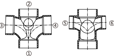
SANITARY TEE W/ LEFT SIDE INLET SANITARY TEE W/ R & L SIDE INLETS DOUBLE SANITARY TEE, W/SIDE INLET
