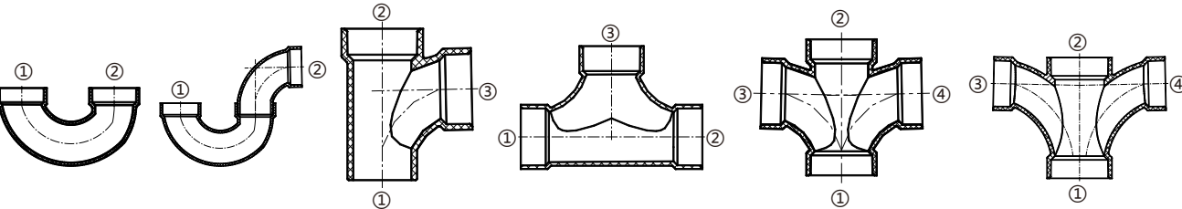
RETURN BEND P-TRAP SANITARY TEE, STREET ELBOW DOUBLE SANITARY TEE DOUBLE FIXTURE FITTING
