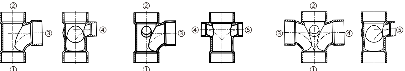
SANITARY TEE W/ LEFT SIDE INLET SANITARY TEE W/ R & L SIDE INLETS DOUBLE SANITARY TEE, W/SIDE INLET
